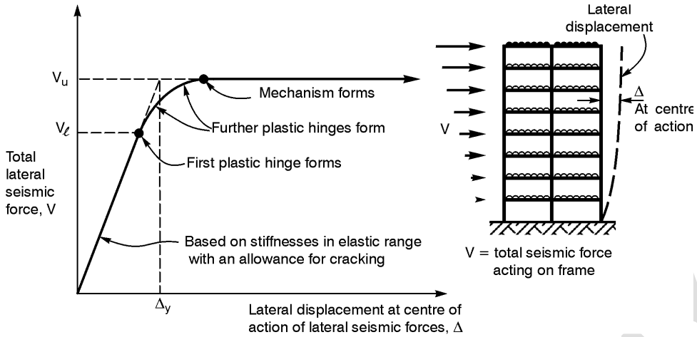
Figure C2.11: Pseudo-nonlinear static pushover analysis with iterative elastic analysis
