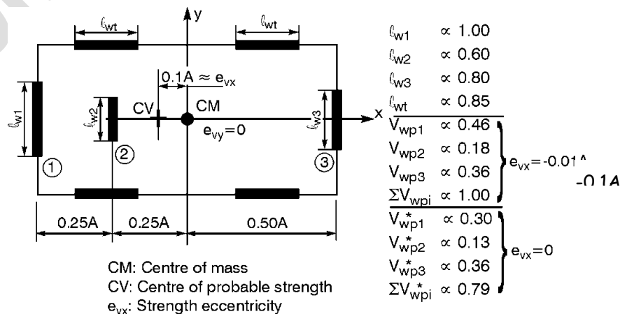
Figure C2F.2: Torsional effects in walled buildings (after Paulay, 2001)
