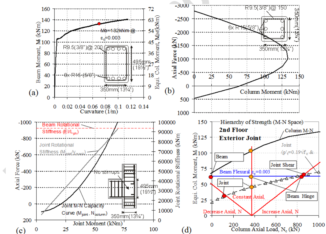
Figure C2A.1: Example of evaluation of element capacity and hierarchy of strength for a non-ductile exterior beam-column joint element as part of a reinforced concrete frame system (Kam, 2010)
