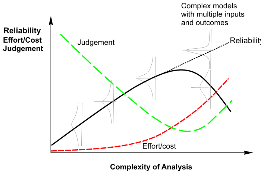
Figure C2.10: Trade-off between reliability, engineering judgement, cost and complexity of structural analysis (modified from Kam and Jury, 2015)
