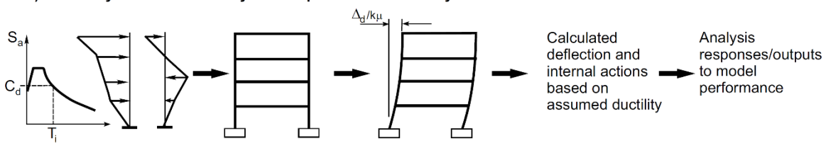
Figure C2.1: Real and modelled responses of buildings to earthquakes
